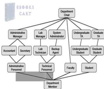
Figure 7: Example of hierarchy of roles for a computer science department.
